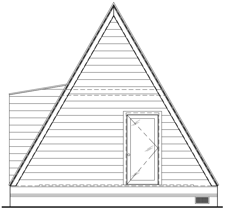
2 REAR ELEVATION 3/16" = 1'-0"
