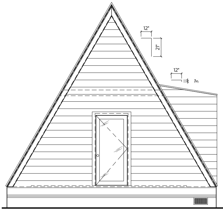
1 FRONT ELEVATION 3/16" = 1'-0"
