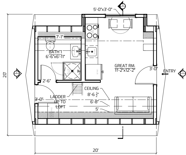
4 1ST LEVEL FLOOR PLAN 1/8" = 1'-0"
