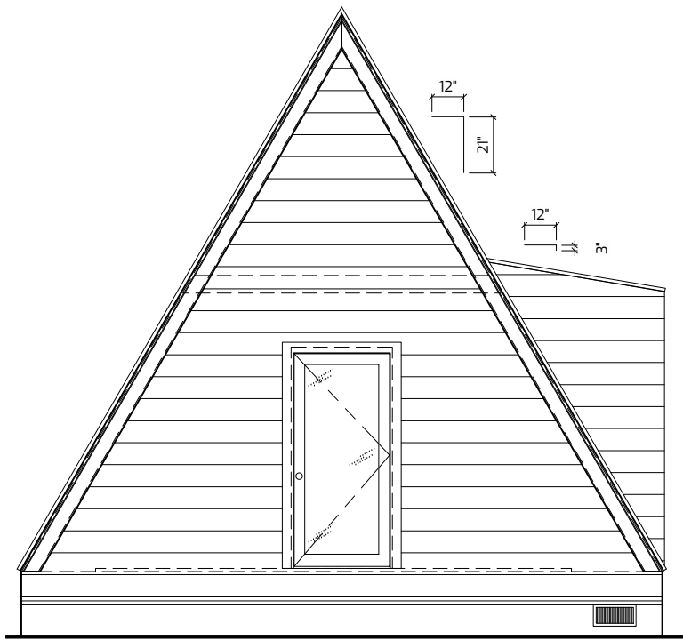
1 FRONT ELEVATION 3/16" = 1'-0"
