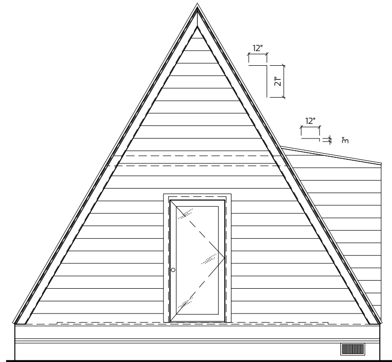
1 FRONT ELEVATION 3/16" = 1'-0"
