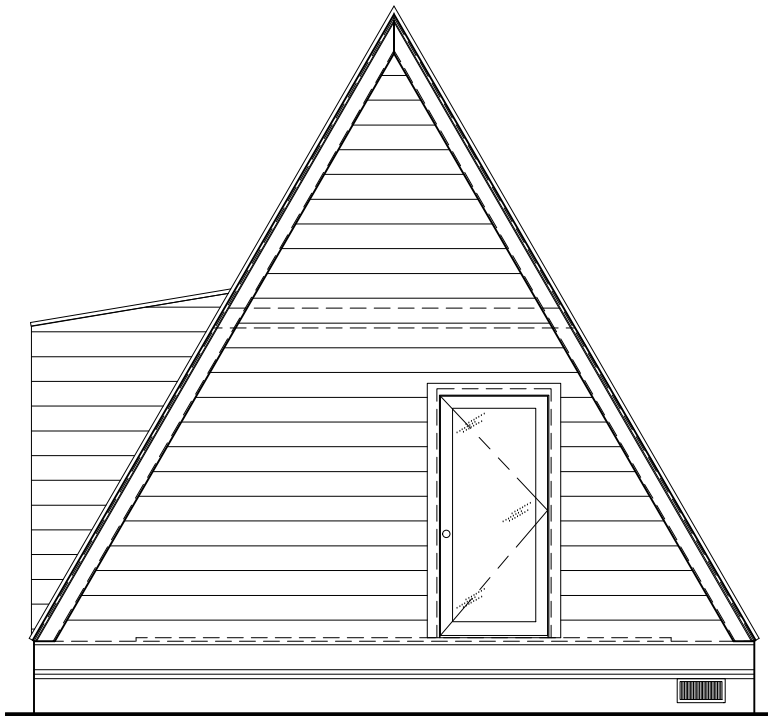
2 REAR ELEVATION 3/16" = 1'-0"
