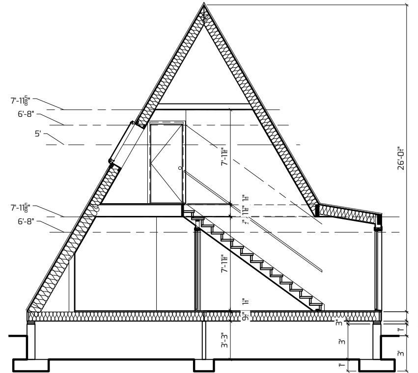
3 SECTION 1/8" = 1'-0"
