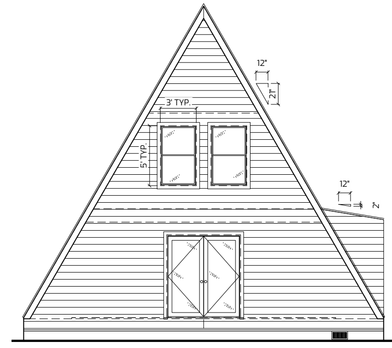
1 FRONT ELEVATION 1/8" = 1'-0"
