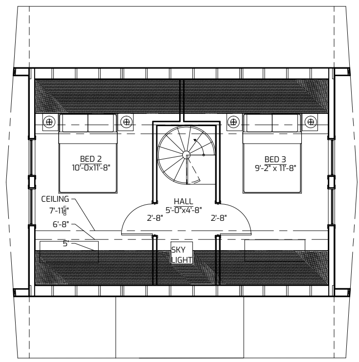
5 2ND LEVEL FLOOR PLAN 1/8" = 1'-0"
