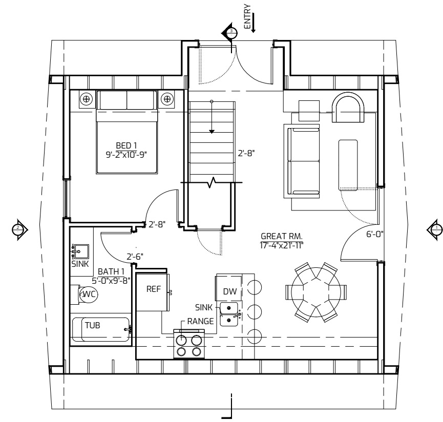
4 1ST LEVEL FLOOR PLAN 1/8" = 1'-0"
