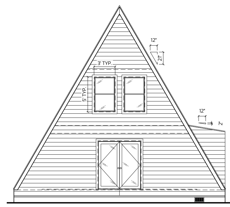
1 FRONT ELEVATION 1/8" = 1'-0"
