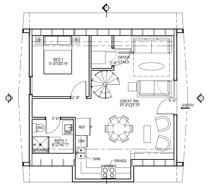
4 1ST LEVEL FLOOR PLAN 1/8" = 1'-0"
