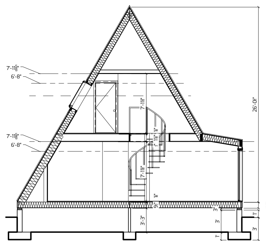
3 SECTION 1/8" = 1'-0"
