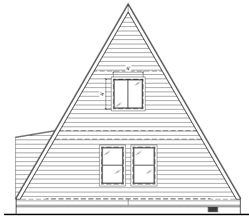
1 REAR ELEVATION 1/8" = 1'-0"
