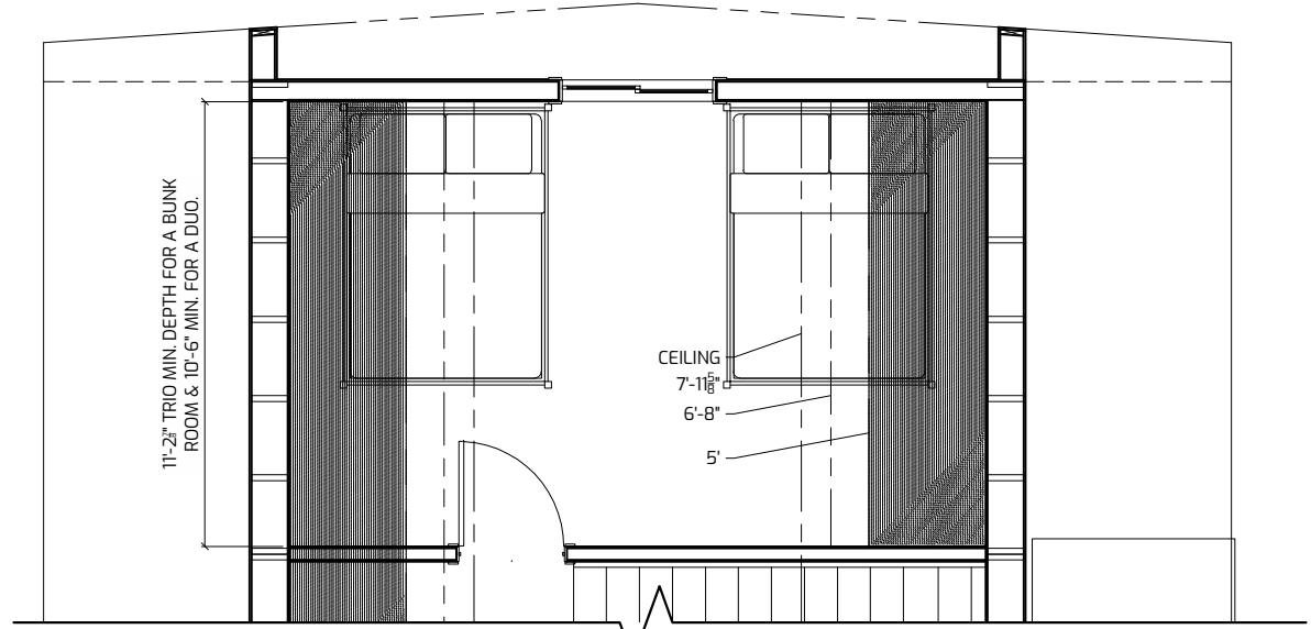
2 TRIO 2ND LEVEL BUNK ROOM PLAN VIEW 3/16" = 1'-0"
