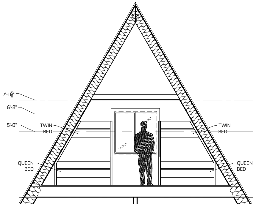
3 TRIO SECTION @ BUNK ROOM 3/16" = 1'-0"
