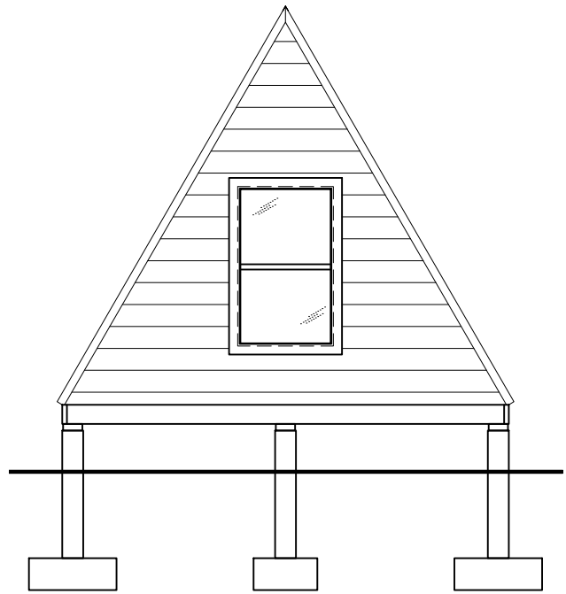
2 REAR ELEVATION NTS
