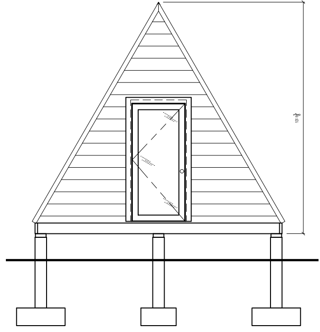
1 FRONT ELEVATION NTS
