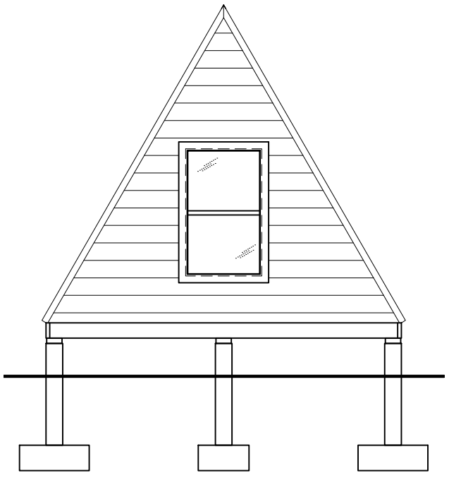
2 REAR ELEVATION NTS
