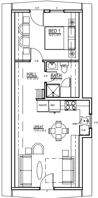
3 FLOOR PLAN NTS
