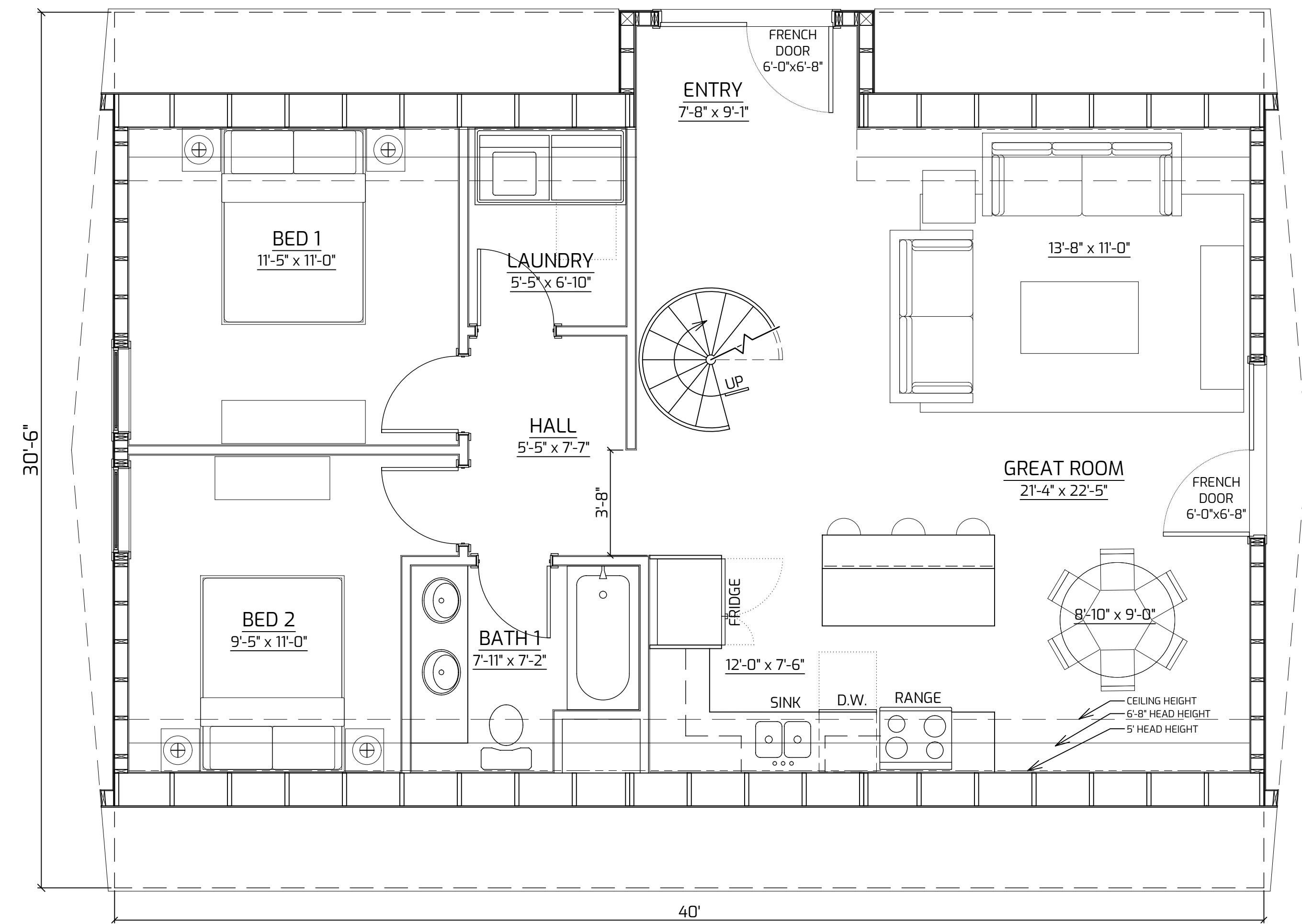
MAIN LEVEL FLOOR PLAN NTS
