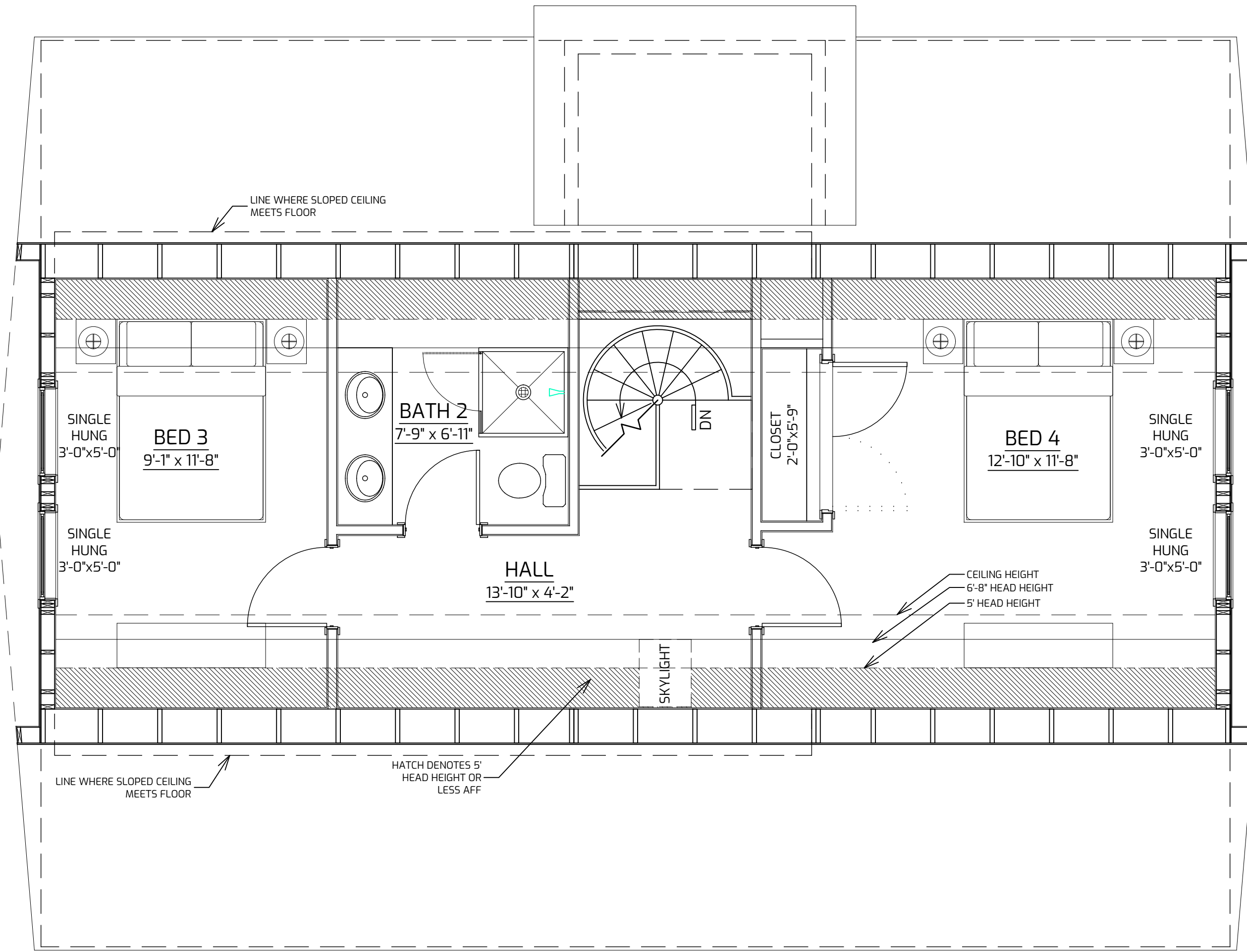
UPPER LEVEL FLOOR PLAN NTS
