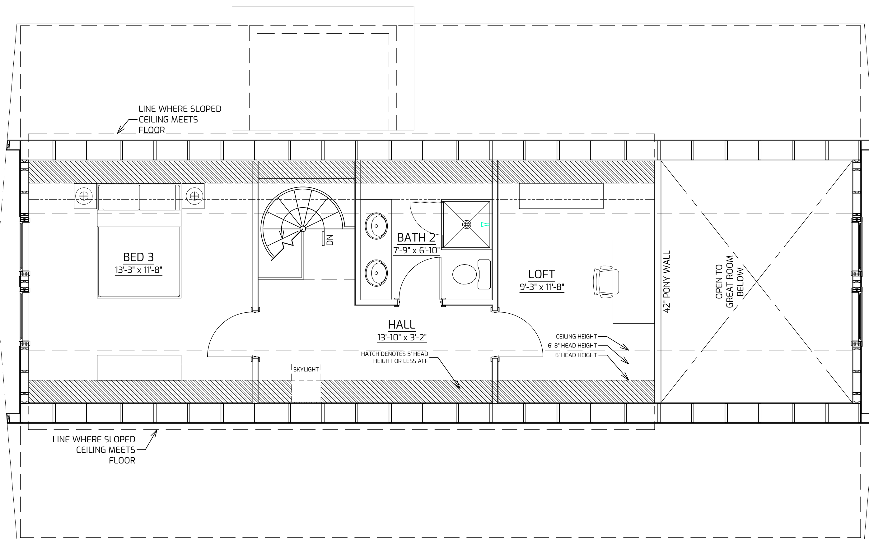
UPPER LEVEL FLOOR PLAN NT5
