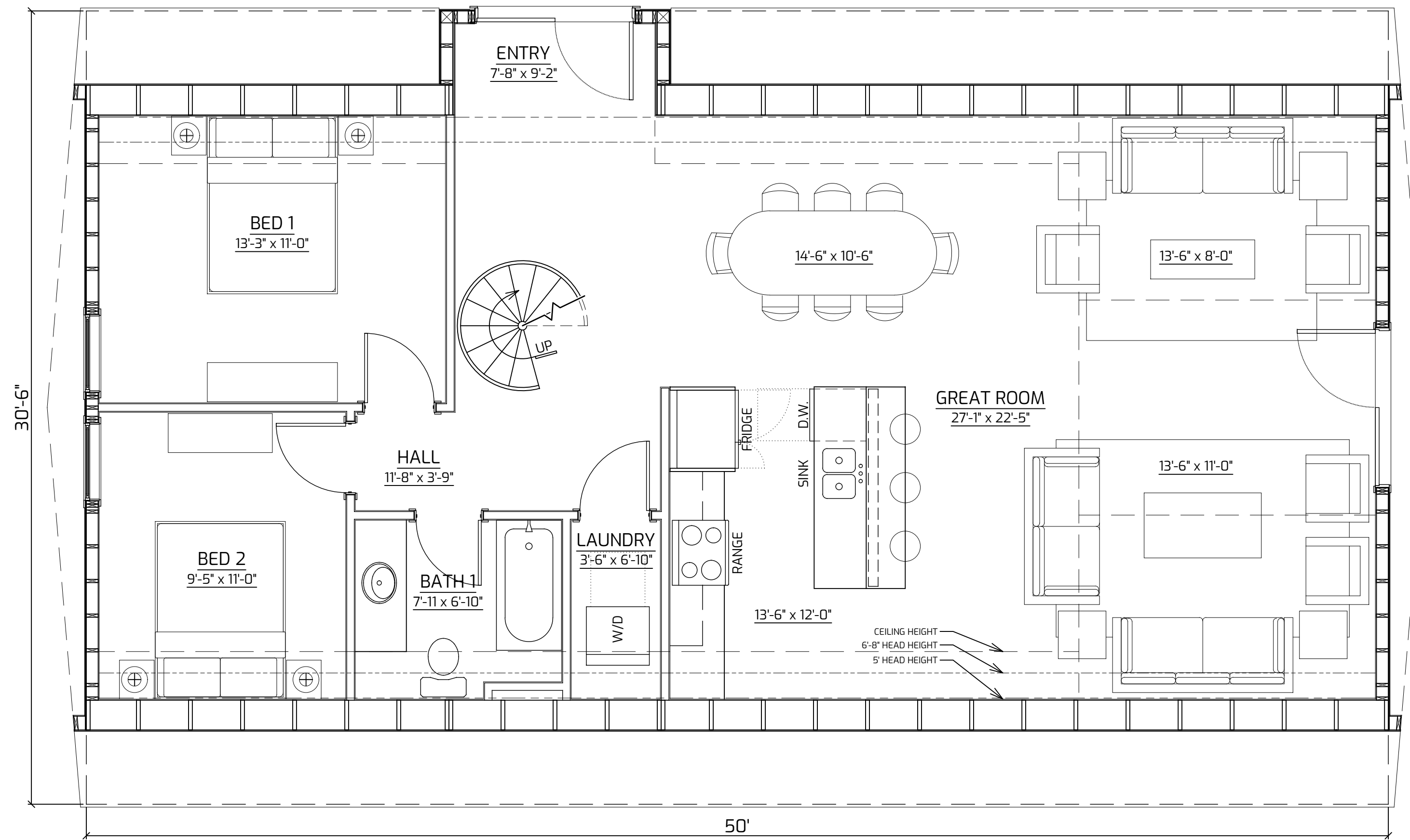
MAIN LEVEL FLOOR PLAN NT5
