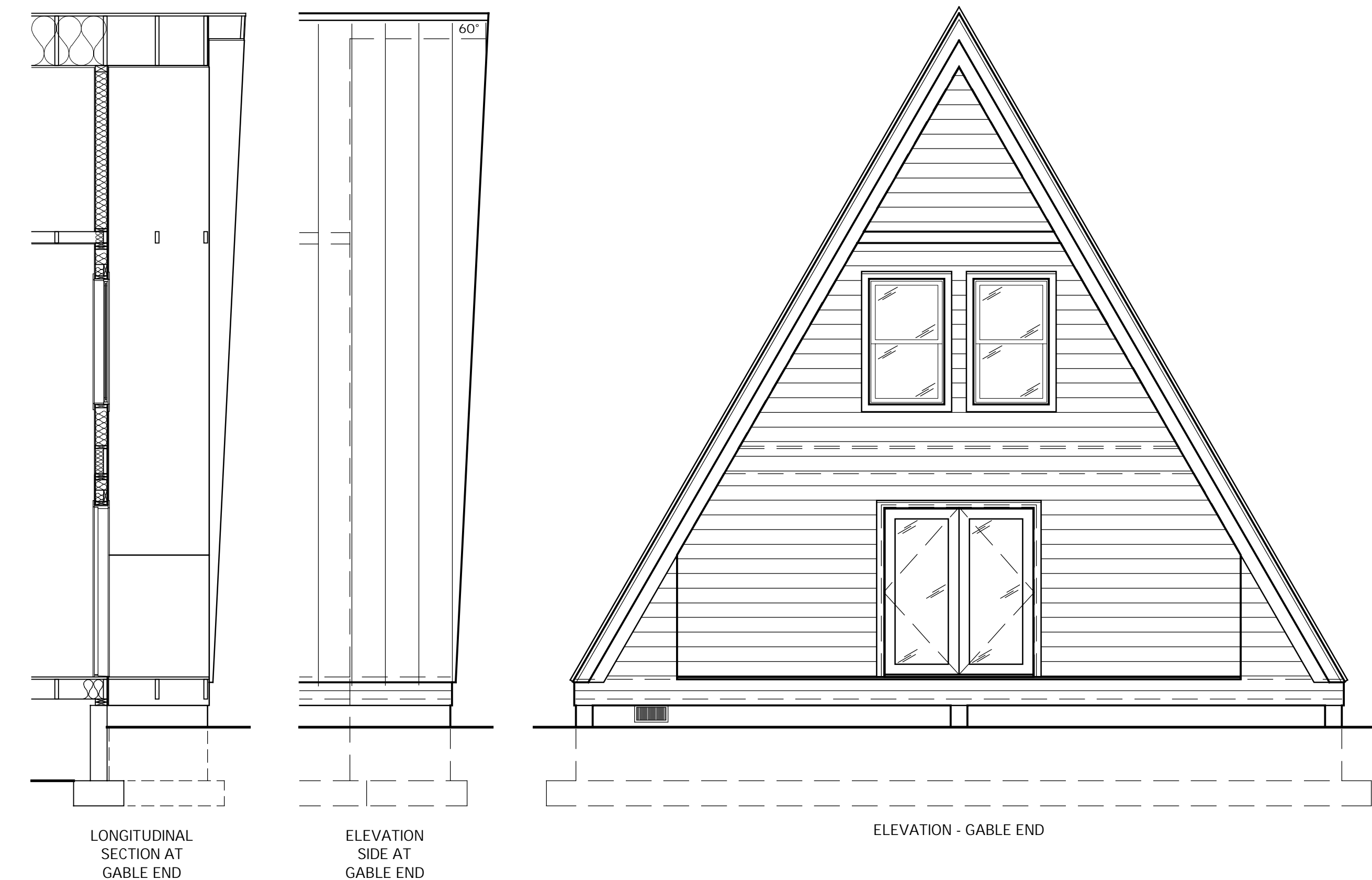
EXTENDED GABLE ROOF W/ MAIN LEVEL DECK
