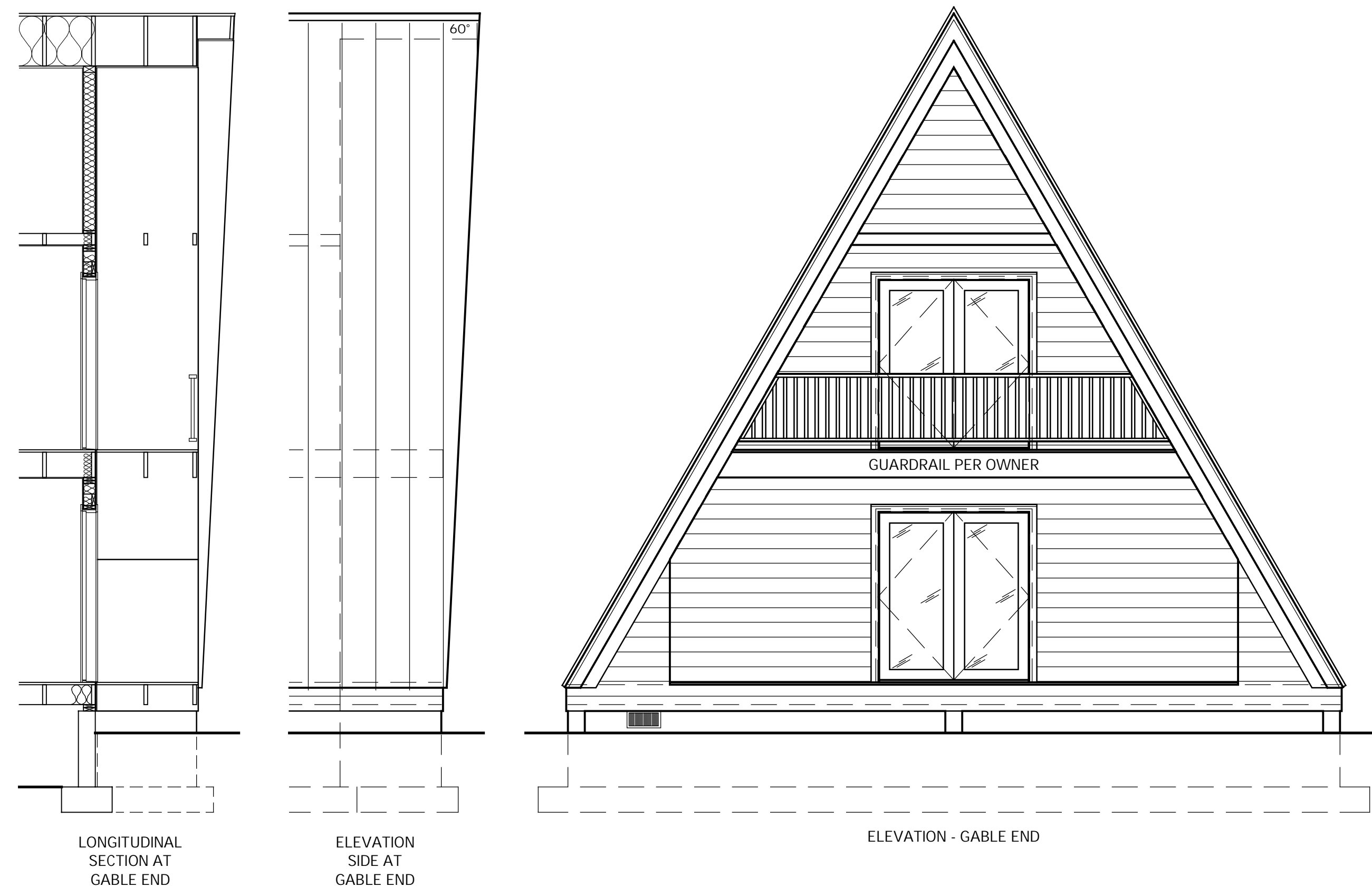
EXTENDED GABLE ROOF W/ MAIN & UPPER LEVEL DECKS
