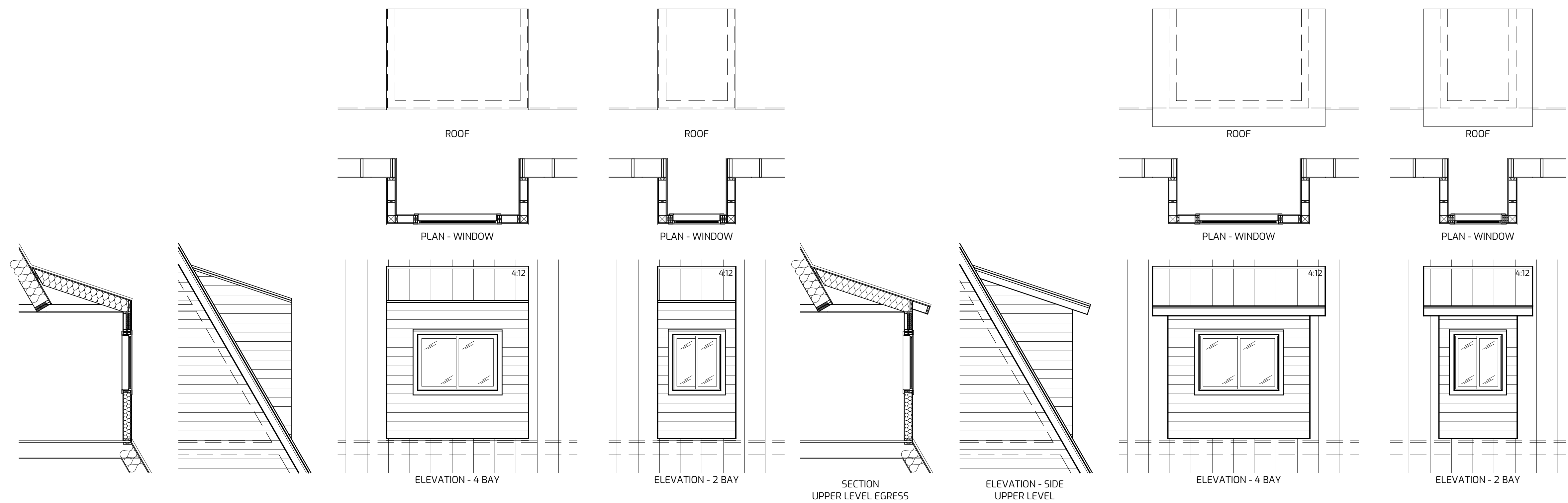
SHED ROOF NO OVERHANG
