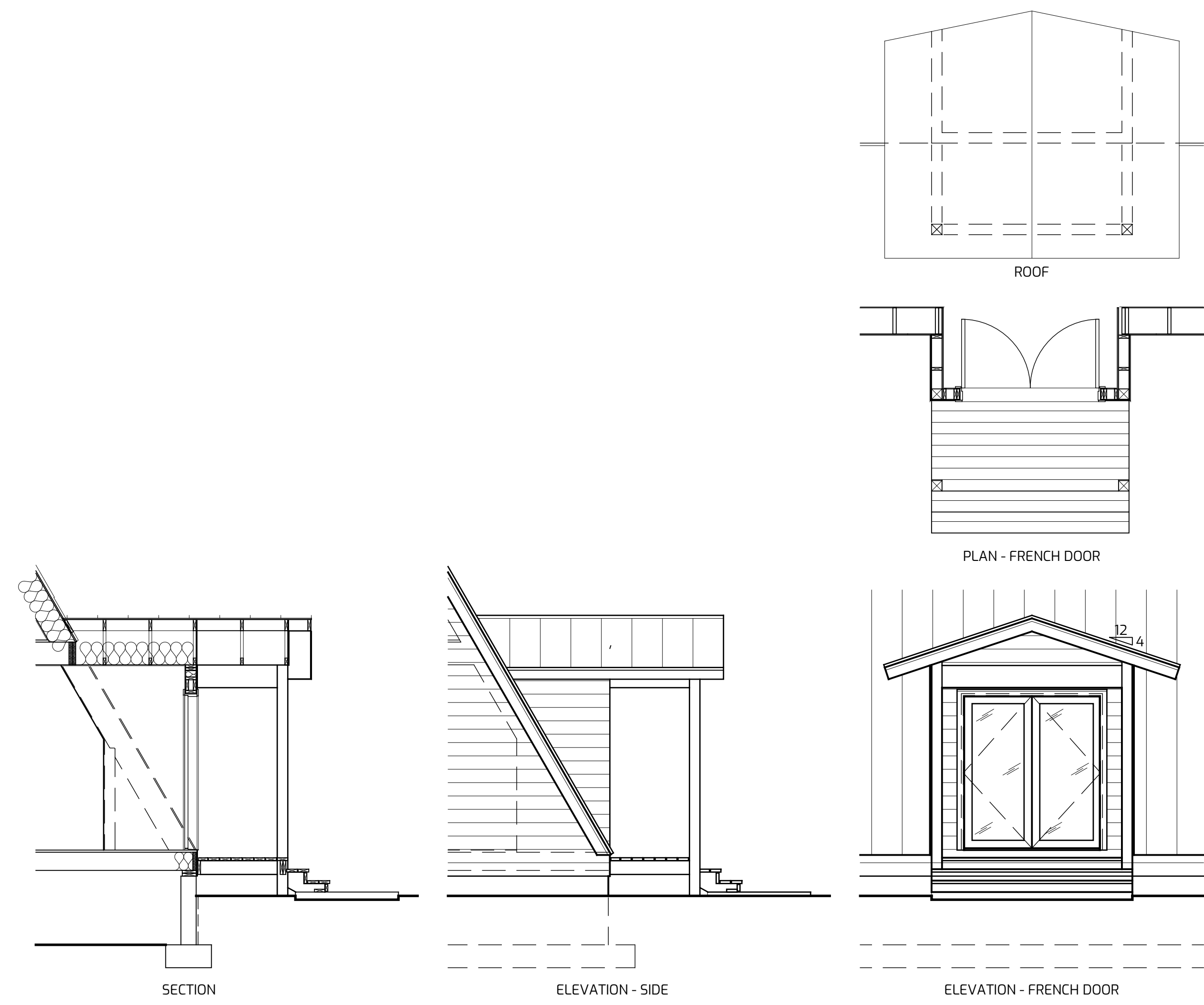
EXTENDED GABLED ROOF W/ DECK
