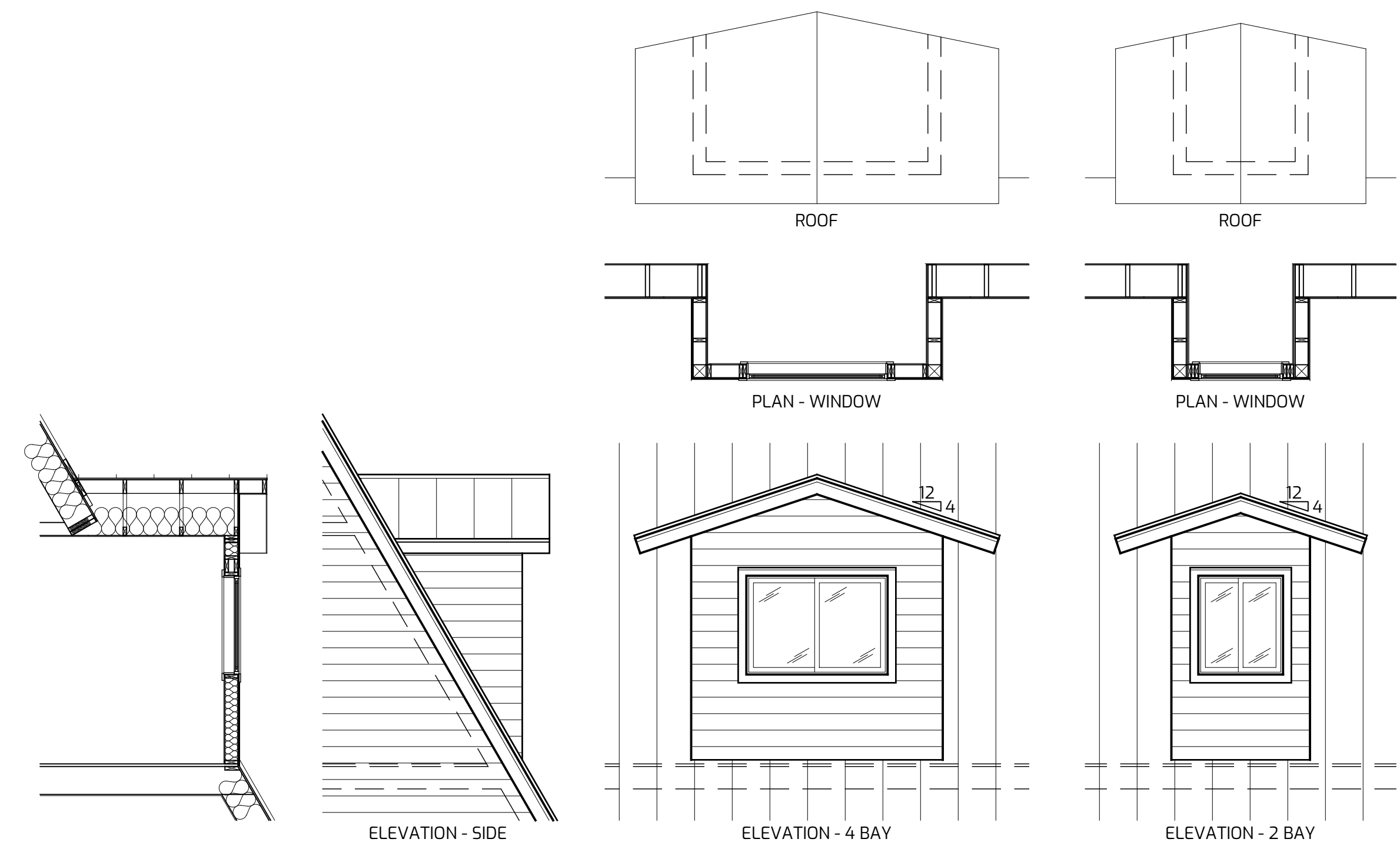
GABLED ROOF
