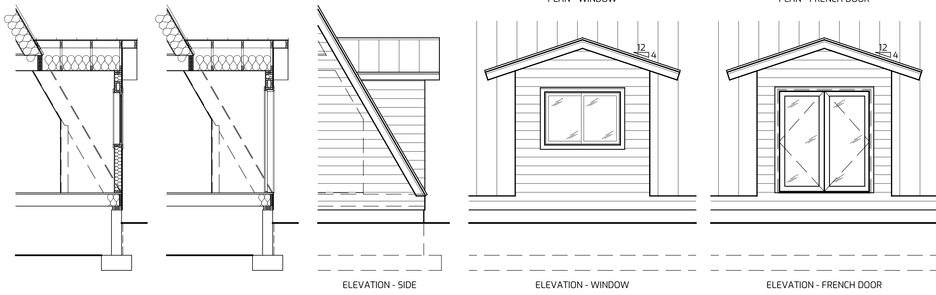
GABLED ROOF
