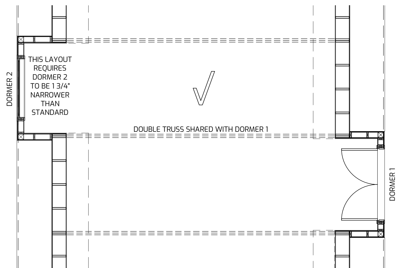
OFFSET - SHARED TRUSS
