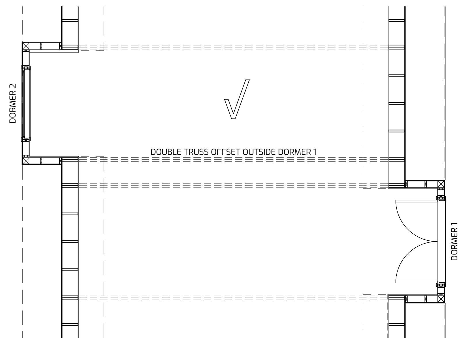
OFFSET - WITH SEPARATION
