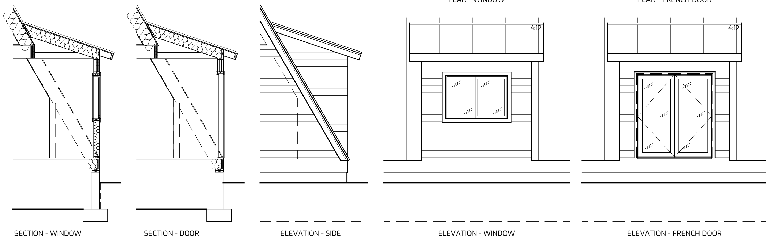
SHED ROOF W/ OVERHANG
