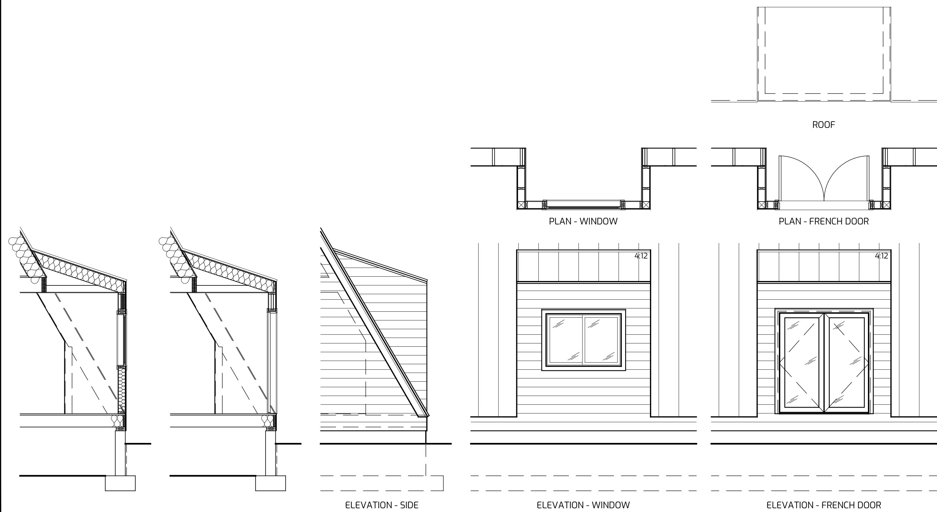
SHED ROOF NO OVERHANG RAFTER TAILS MUST BE CUT OFF ON SITE
