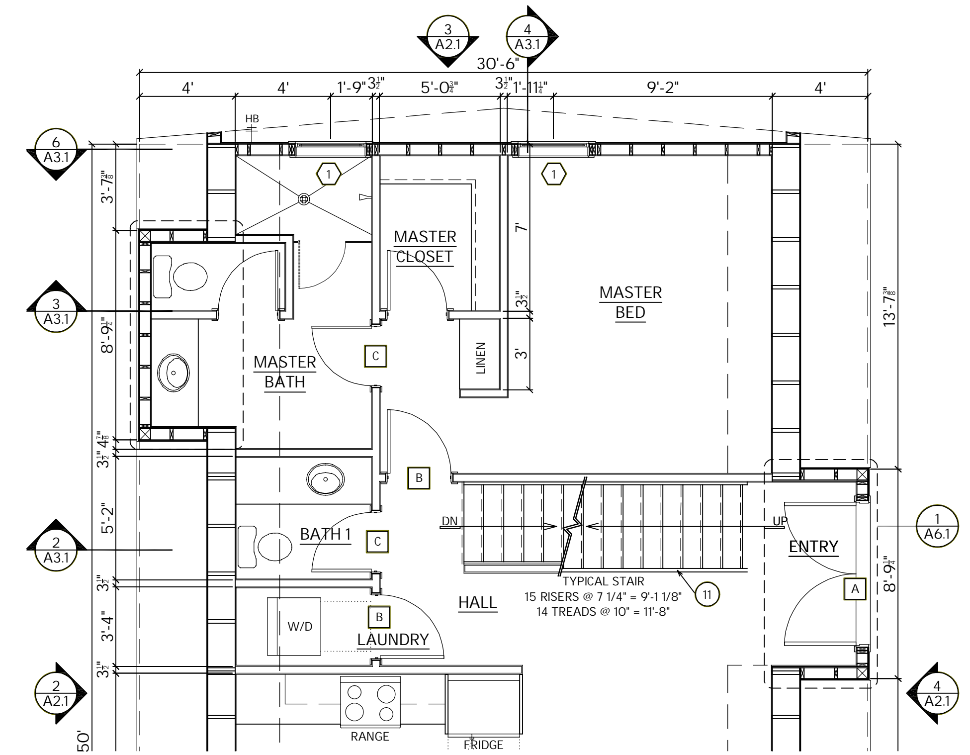
2 TRIO 150 MASTER BEDROOM OPTION "A" W/ DORMER 1/4" = 1'-0"
