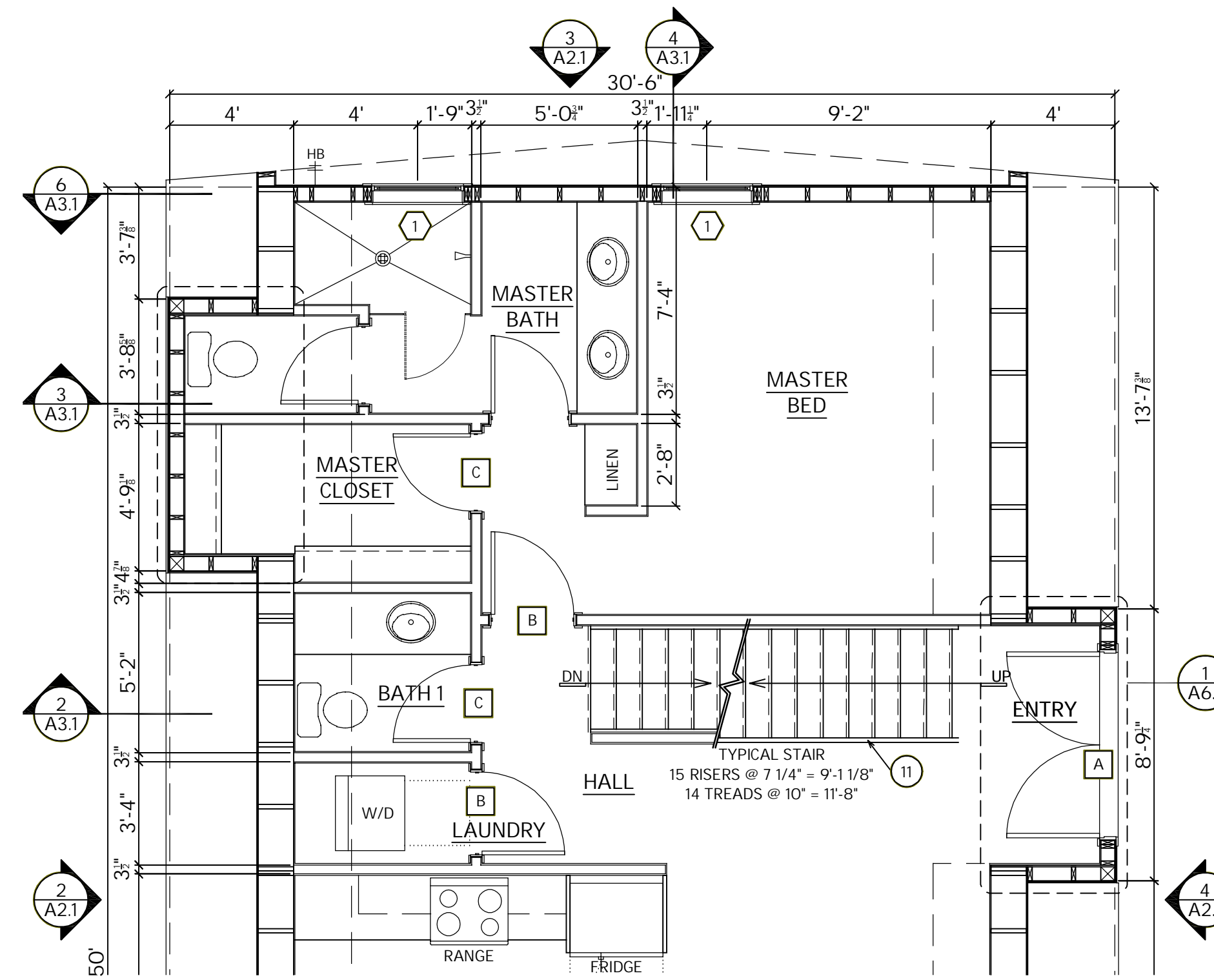
4 TRIO 150 MASTER BEDROOM OPTION "B" W/ DORMER 1/4" = 1'-0"
