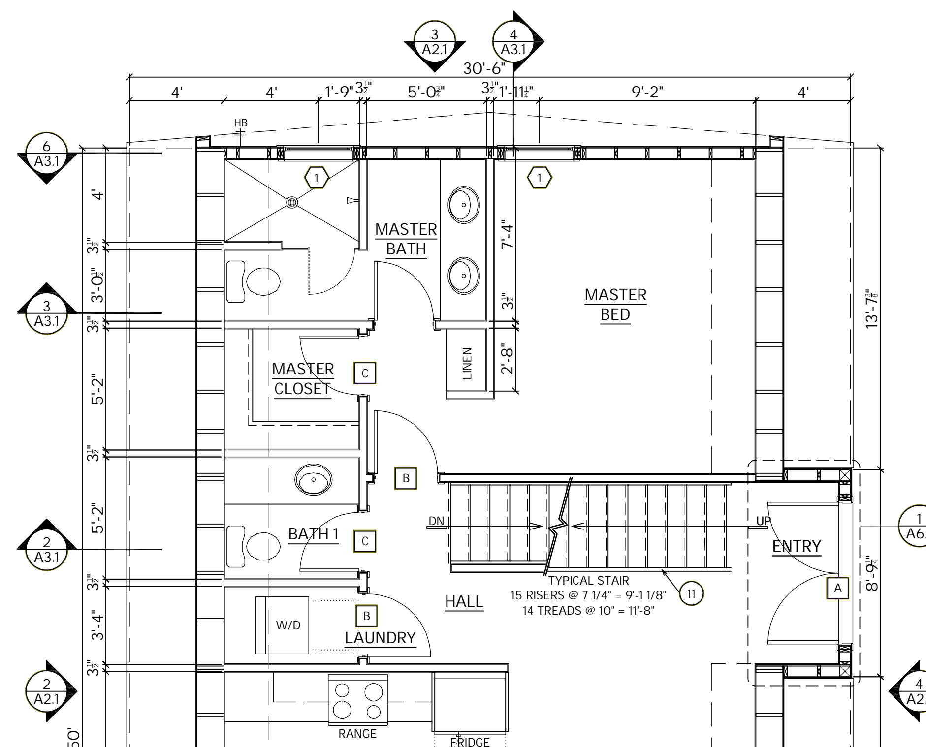
3 TRIO 150 MASTER BEDROOM OPTION "B" 1/4" = 1'-0"
