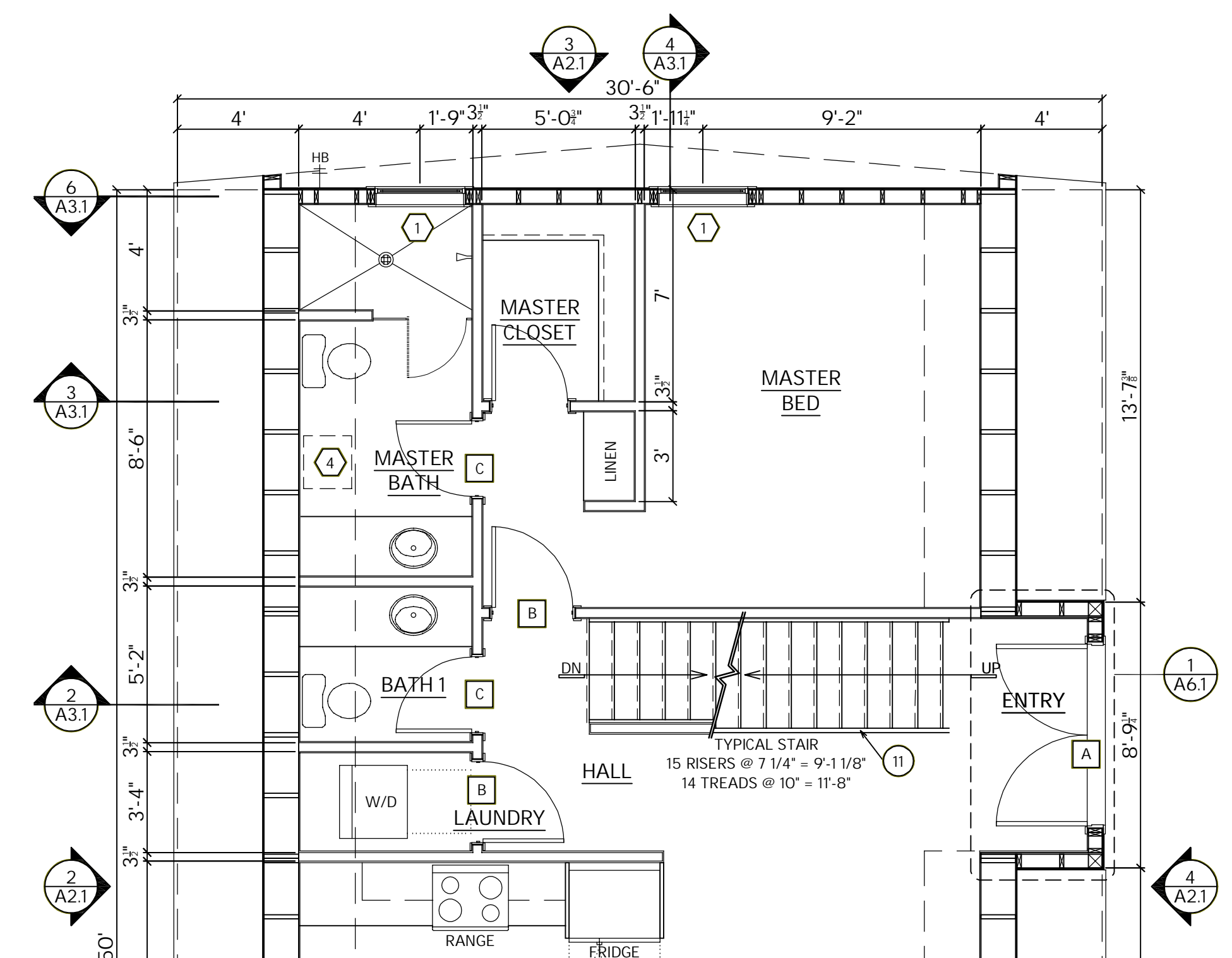
1 TRIO 150 MASTER BEDROOM OPTION "A" 1/4" = 1'-0"
