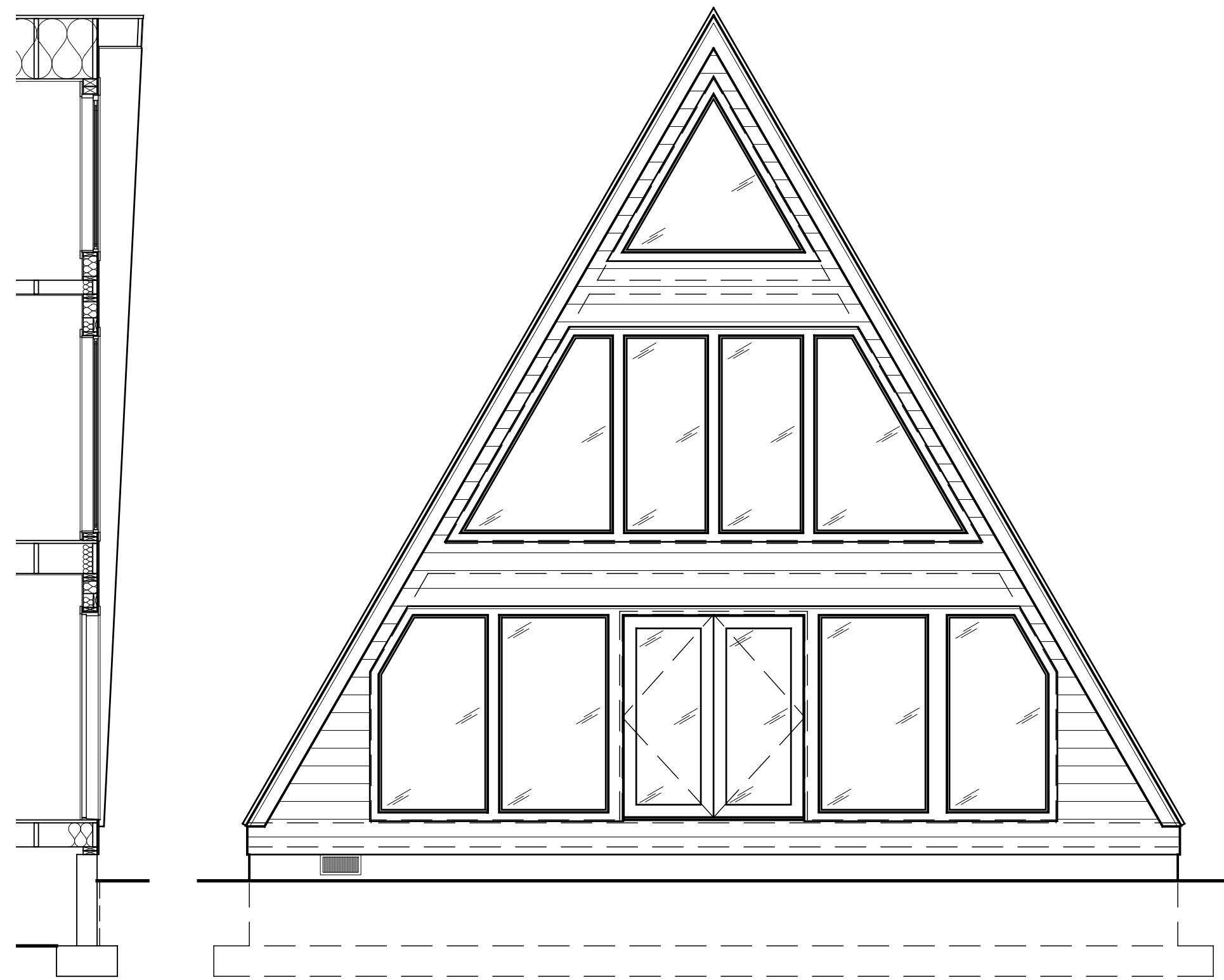
EUROPEAN W/ TRIANGLE WINDOW
