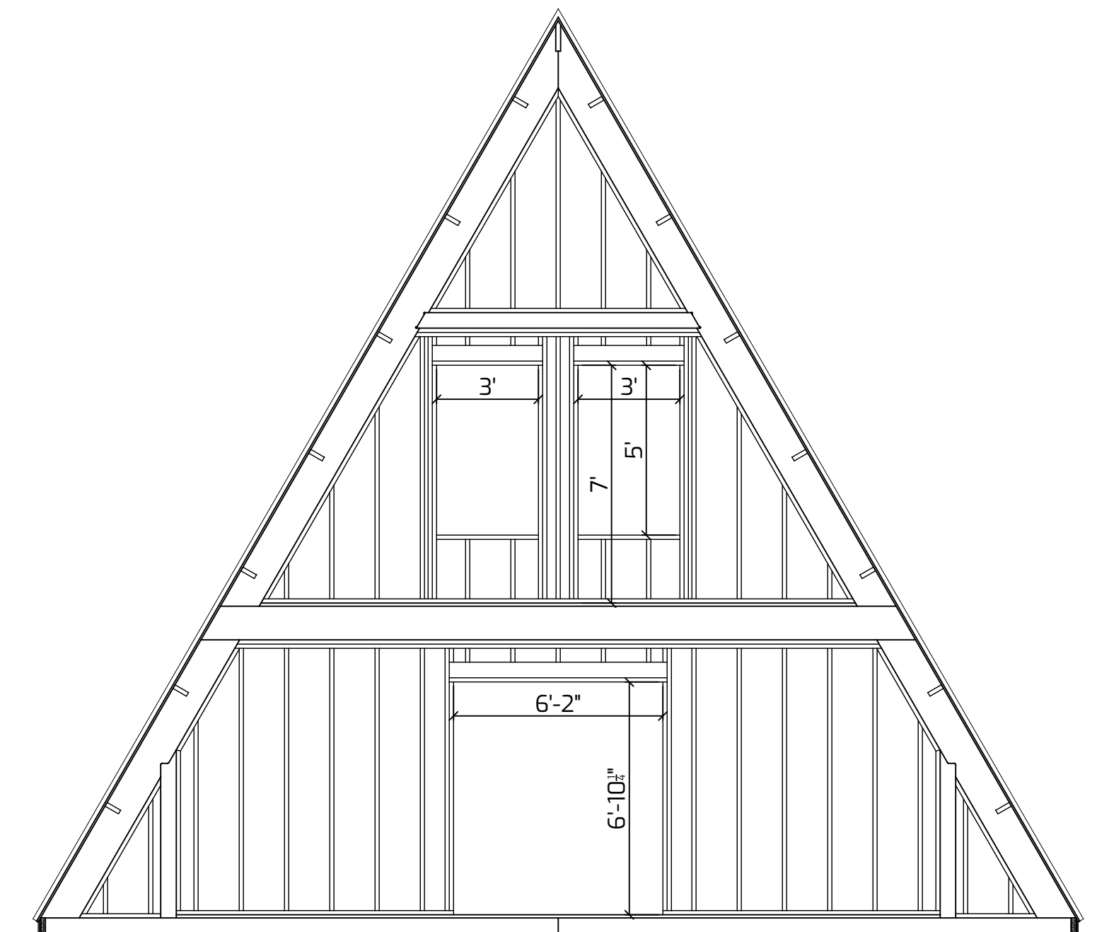
GABLE FRAMING
