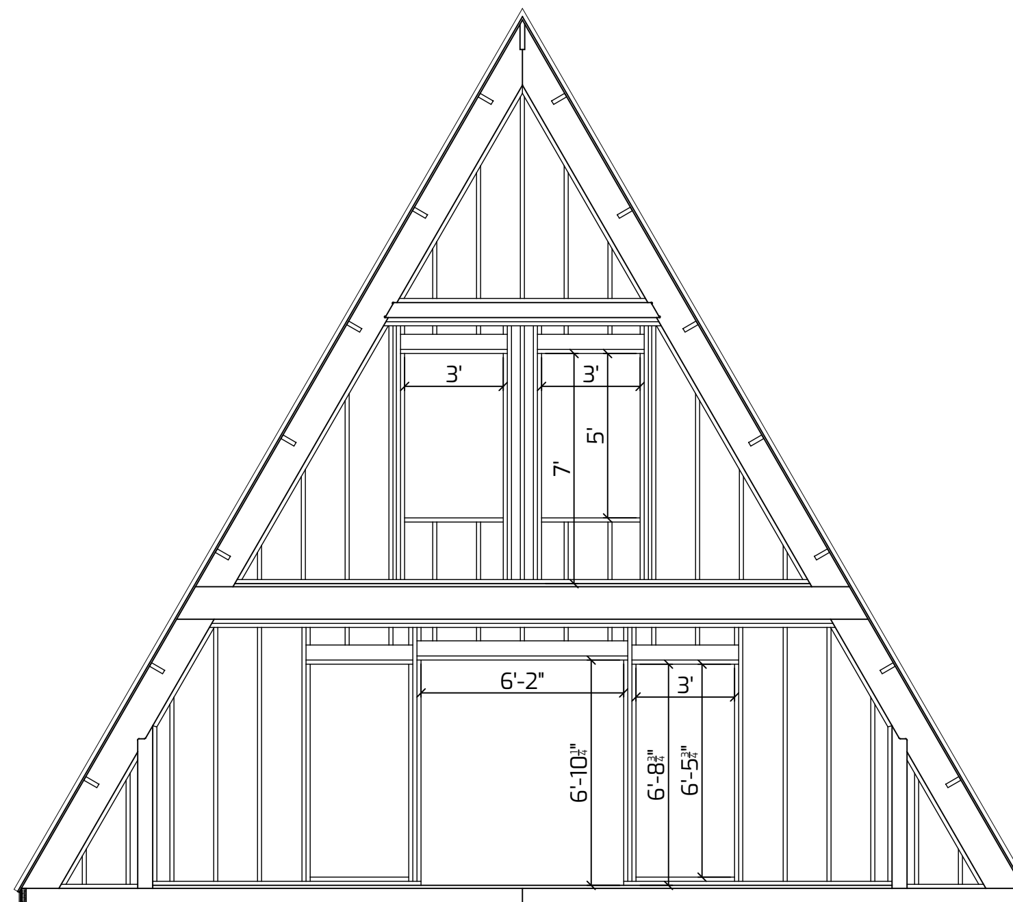
GABLE FRAMING
