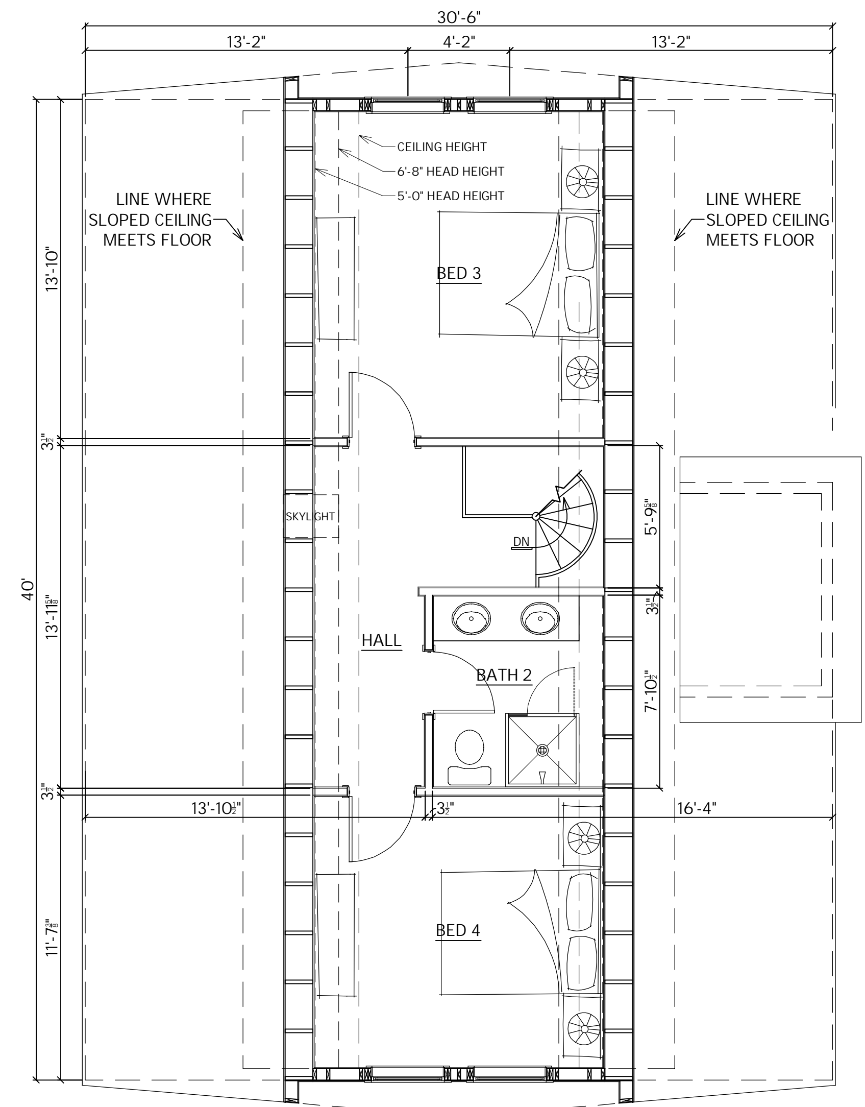
UPPER LEVEL FLOOR PLAN NOT TO SCALE
