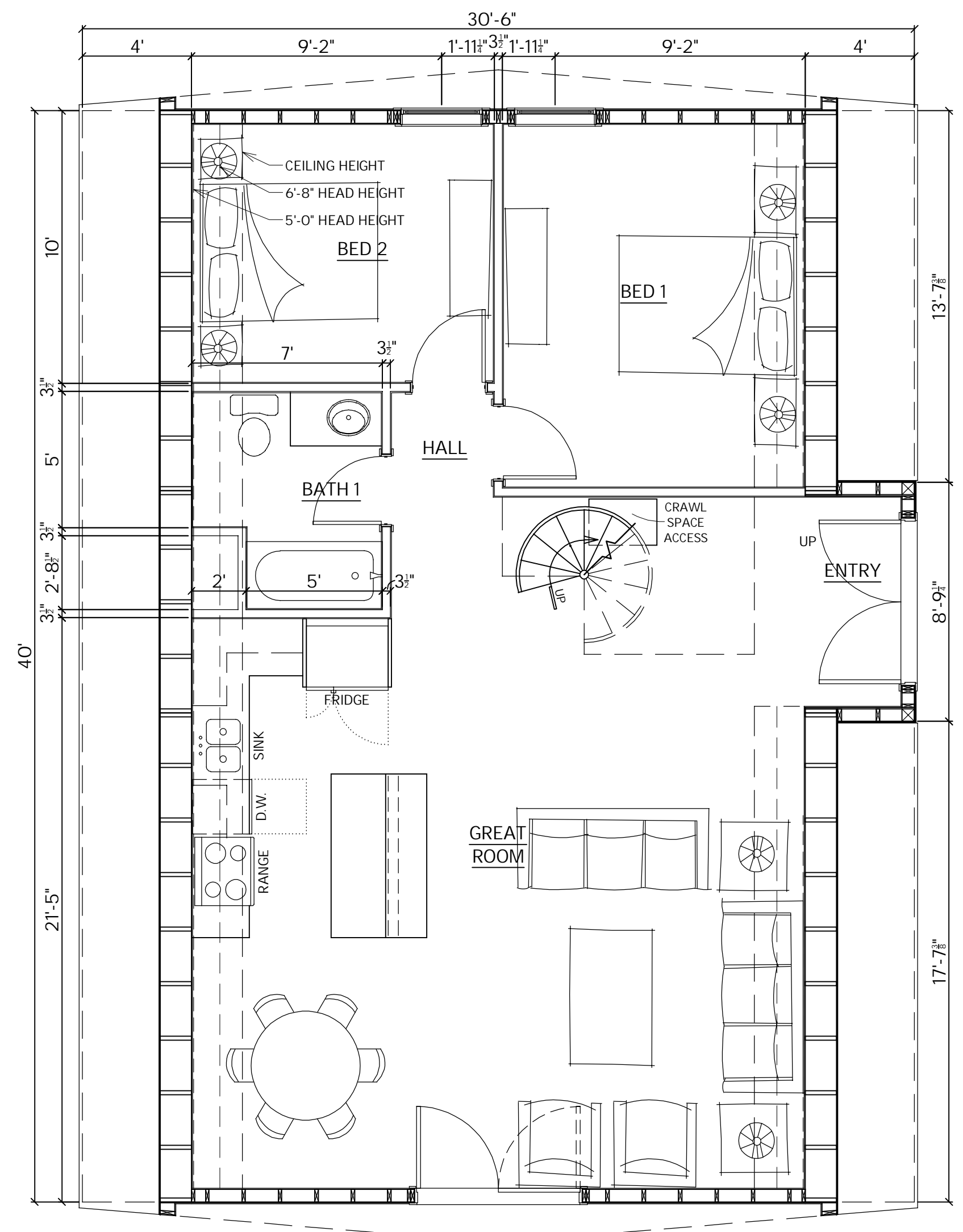
MAIN LEVEL FLOOR PLAN NOT TO SCALE
