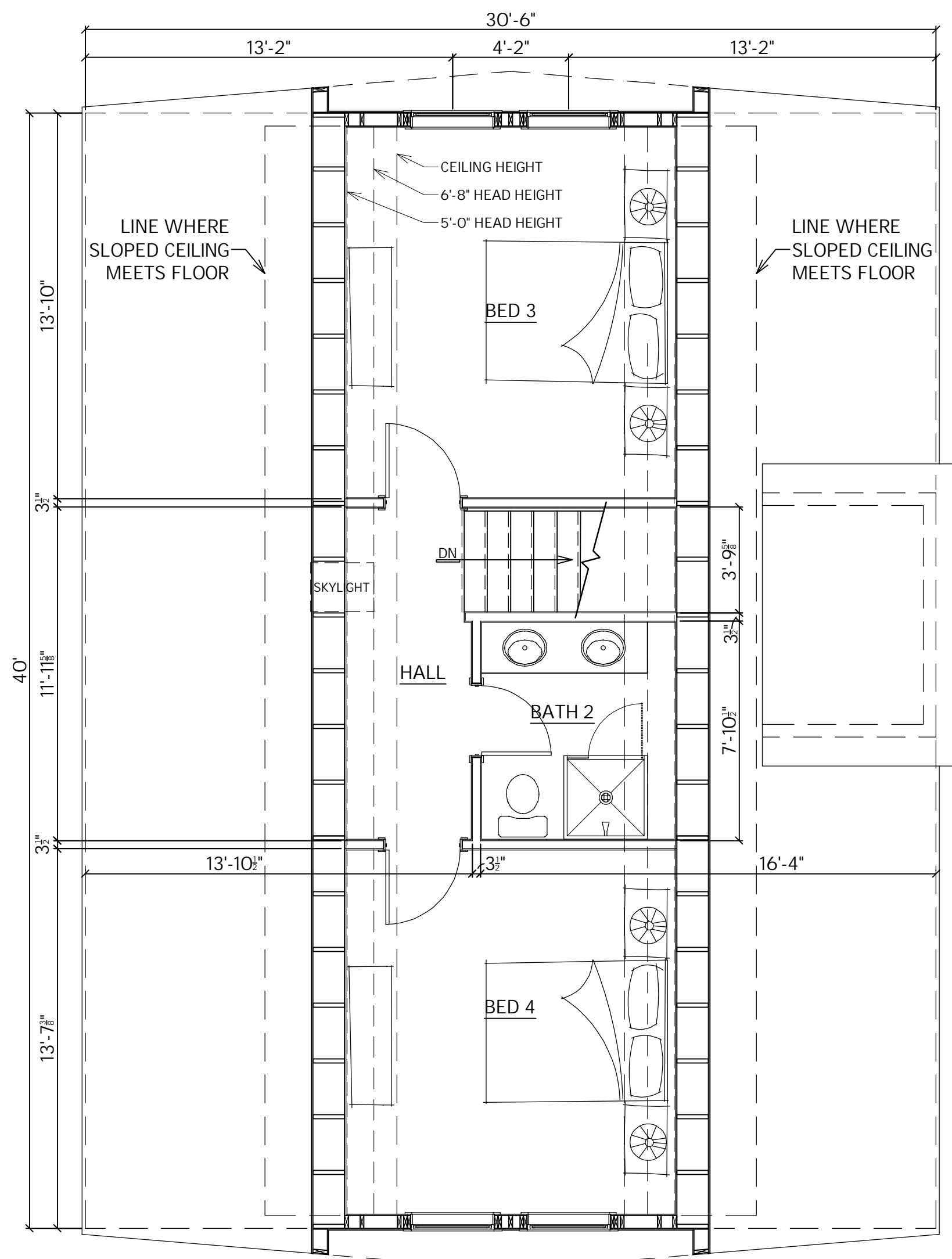
UPPER LEVEL FLOOR PLAN NOT TO SCALE
