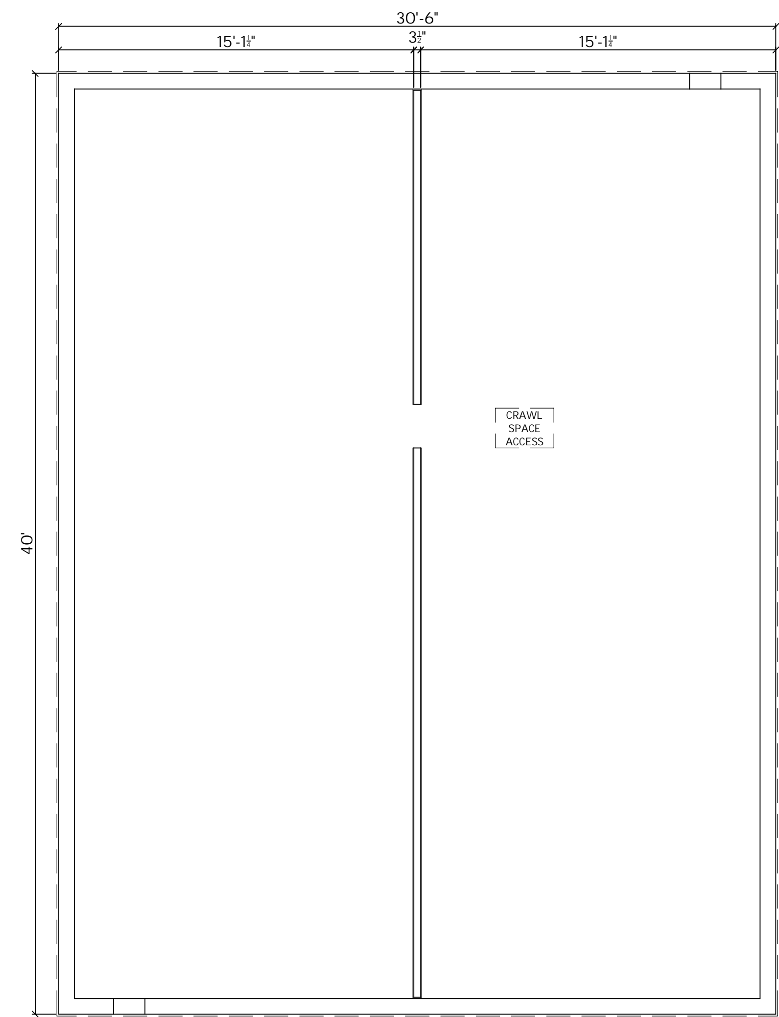
CRAWL SPACE PLAN NOT TO SCALE
