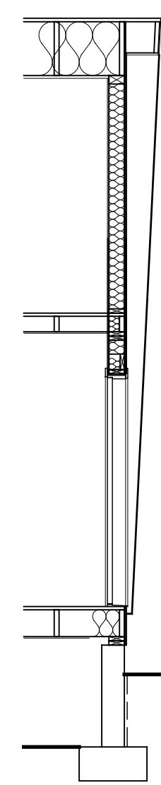
LONGITUDINAL SECTION AT GABLE END
