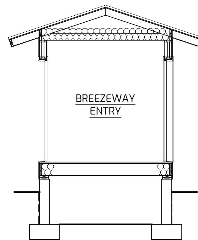
CROSS SECTION
