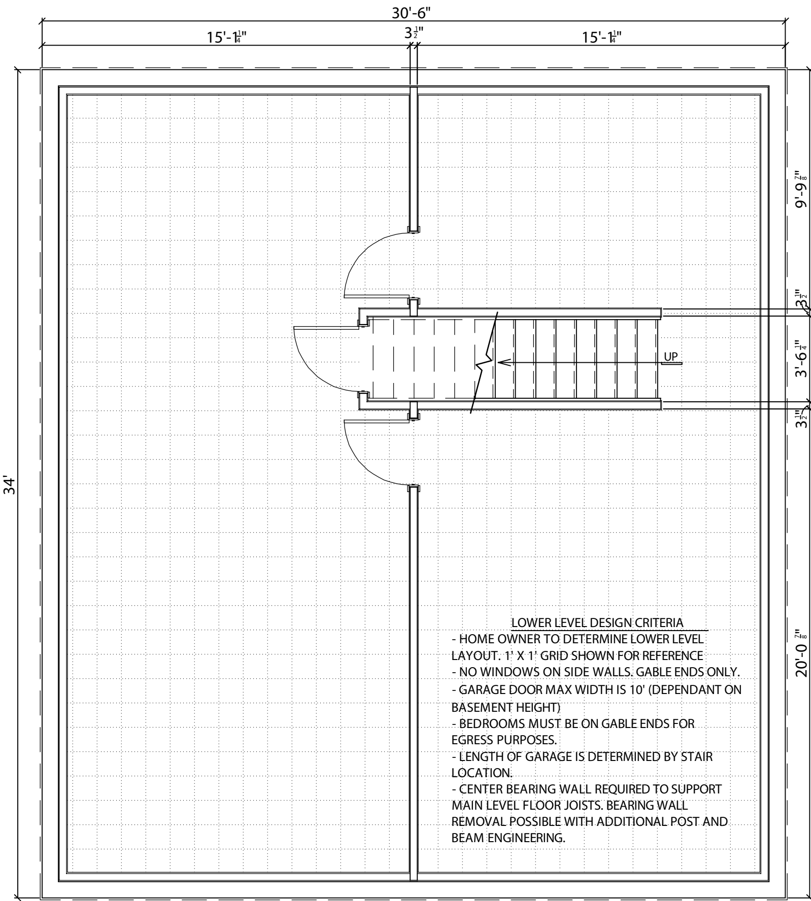
LOWER LEVEL FLOOR PLAN NOT TO SCALE
