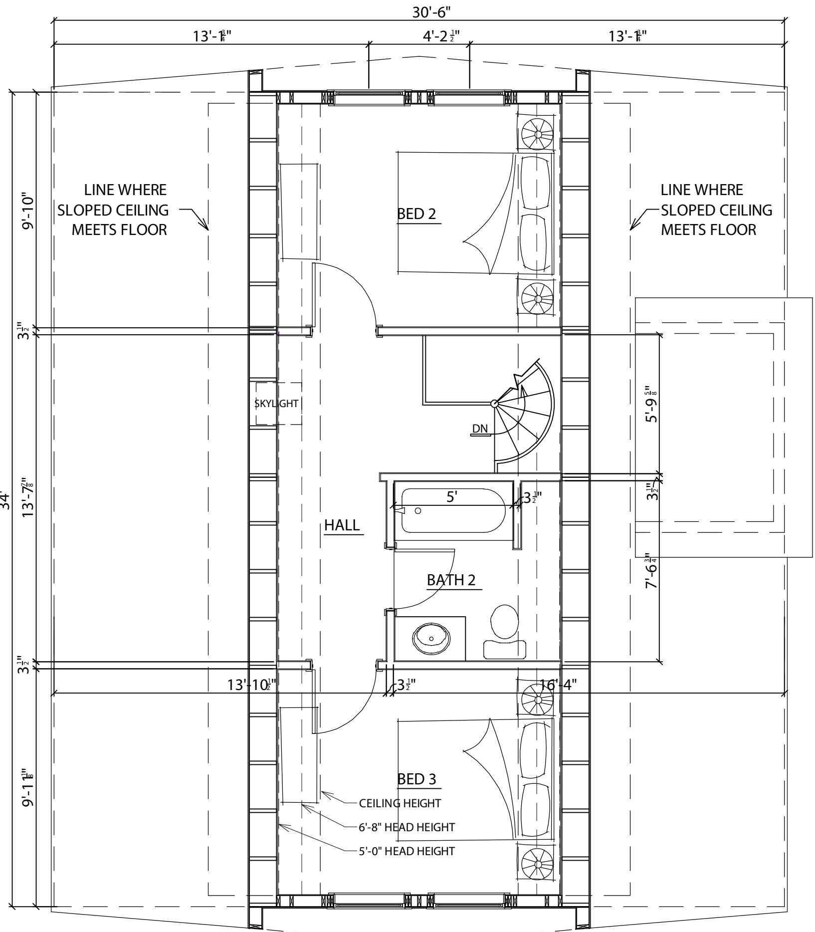
UPPER LEVEL FLOOR PLAN NOT TO SCALE
