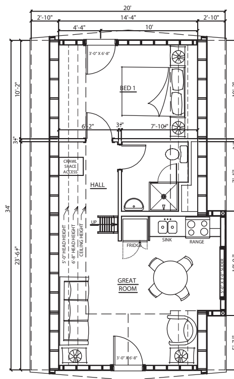
MAIN LEVEL FLOOR PLAN NOT TO SCALE
