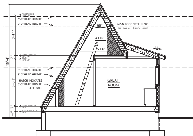
BUILDING SECTION NOT TO SCALE
