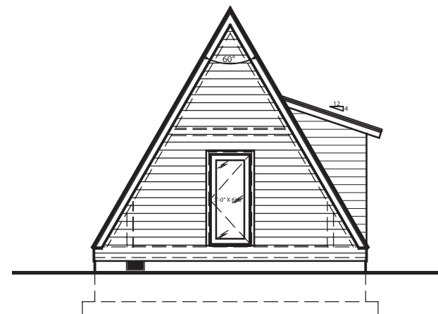
FRONT ELEVATION NOT TO SCALE
