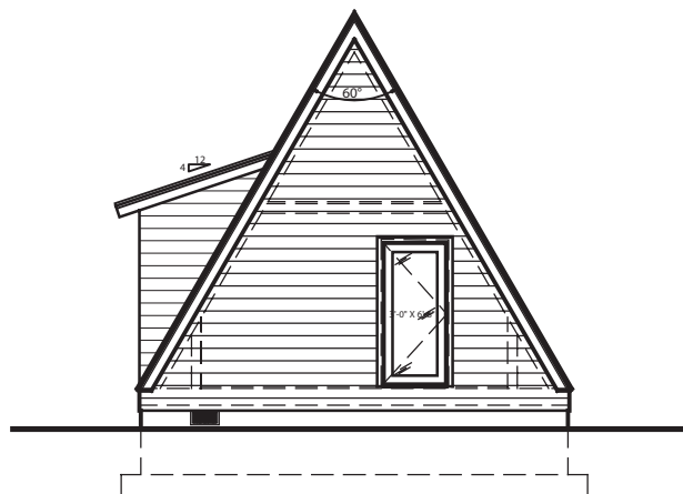
REAR ELEVATION NOT TO SCALE
