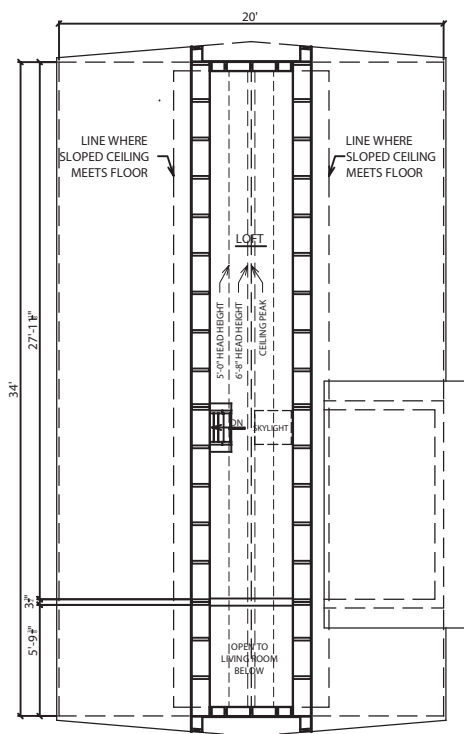
UPPER LEVEL FLOOR PLAN NOT TO SCALE
