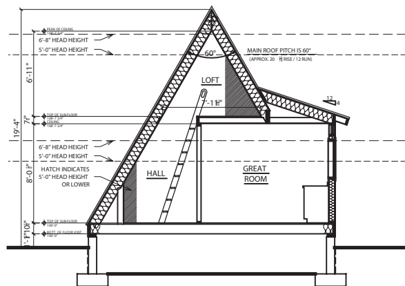
BUILDING SECTION NOT TO SCALE
