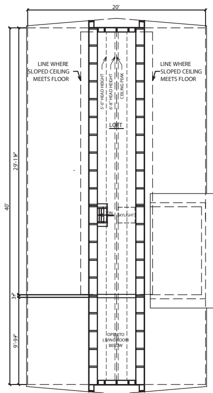
UPPER LEVEL FLOOR PLAN NOT TO SCALE
