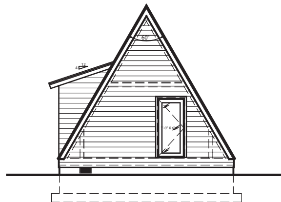
REAR ELEVATION NOT TO SCALE
