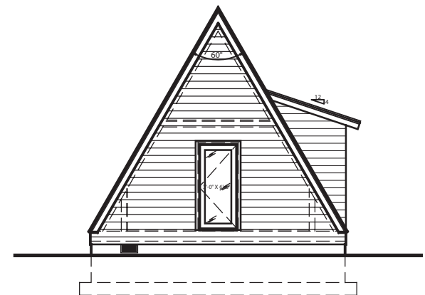
FRONT ELEVATION NOT TO SCALE
