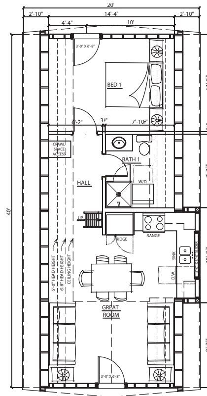
MAIN LEVEL FLOOR PLAN NOT TO SCALE
