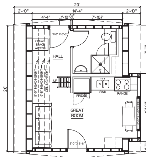
MAIN LEVEL FLOOR PLAN NOT TO SCALE
