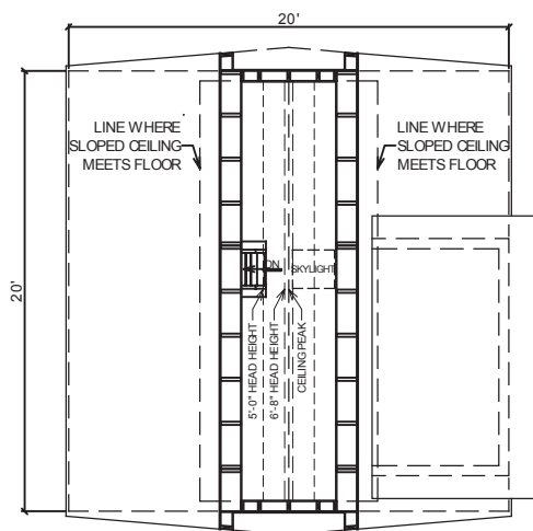
UPPER LEVEL FLOOR PLAN NOT TO SCALE
