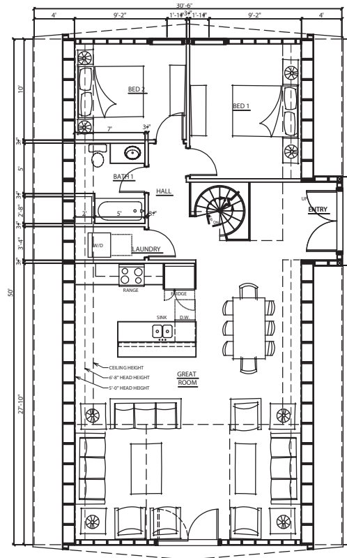
MAIN LEVEL FLOOR PLAN NOT TO SCALE
