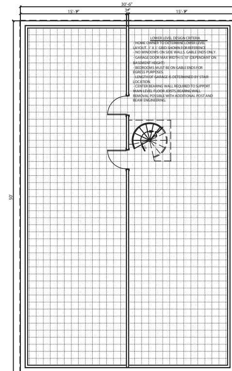
CRAWL SPACE PLAN NOT TO SCALE
