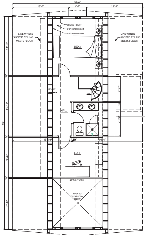
UPPER LEVEL FLOOR PLAN NOT TO SCALE
