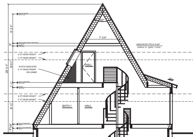
BUILDING CROSS SECTION NOT TO SCALE
